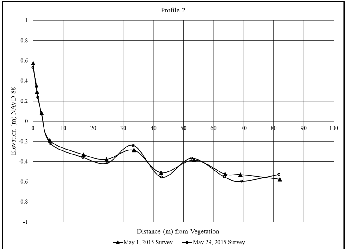
Figure 22. Transect survey data for Profile 2, Alabama Port, Alabama.
