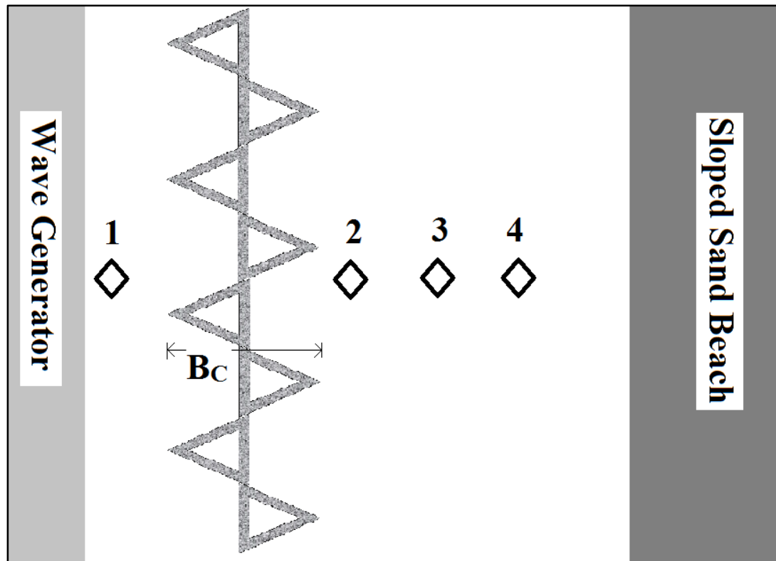
Figure 6. Plan view of the modeled ReefBLK SM breakwater configuration. The crest width measurement and gage placement locations for the ReefBLK SM testing are defined.
