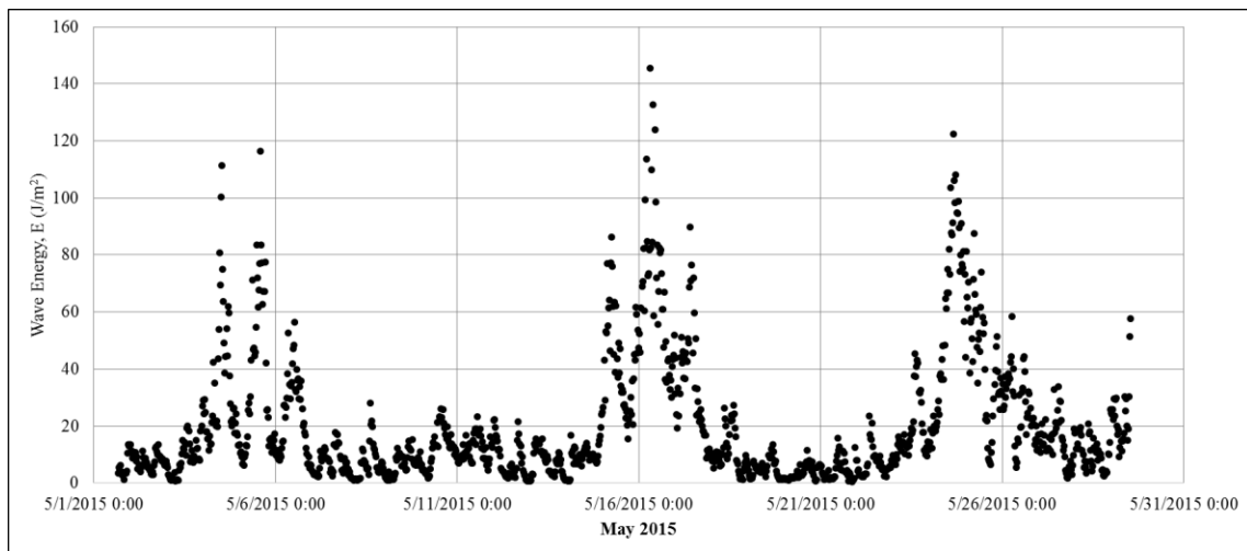
Figure 18. The wave energy record for Sensor 3 at Alabama Port, Alabama during May 2015.
