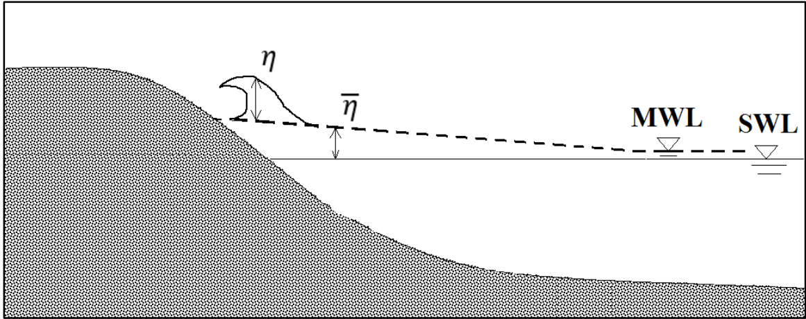
Figure 2. An illustration of standard water level terminology and a definition sketch of wave setup on a shoreline absent of any nearshore structures.
